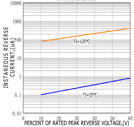
FIG.4-TYPICAL REVERSE CHARACTERISTICS
